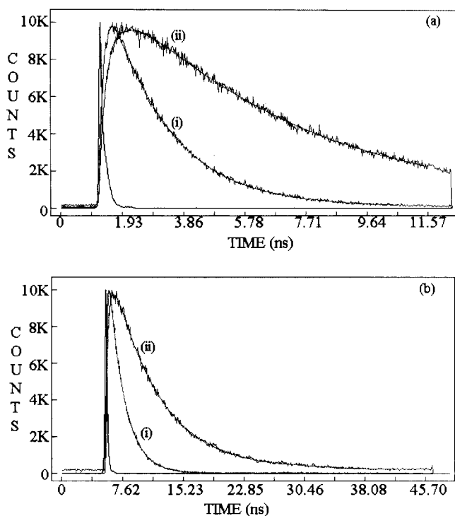
Figure 7. Fluorescence decay of 5 \times 10^{-5} M 1-naphthol in 90% methanol/water (v/v) (a) resolution = 0.0244 ns/ch, (i) \lambda_{em} = 360 nm, (ii) \lambda_{em} = 460 nm; (b) resolution = 0.0952 ns/ch, (i) \lambda_{em} = 360 nm, (ii) \lambda_{em} = 460 nm.
